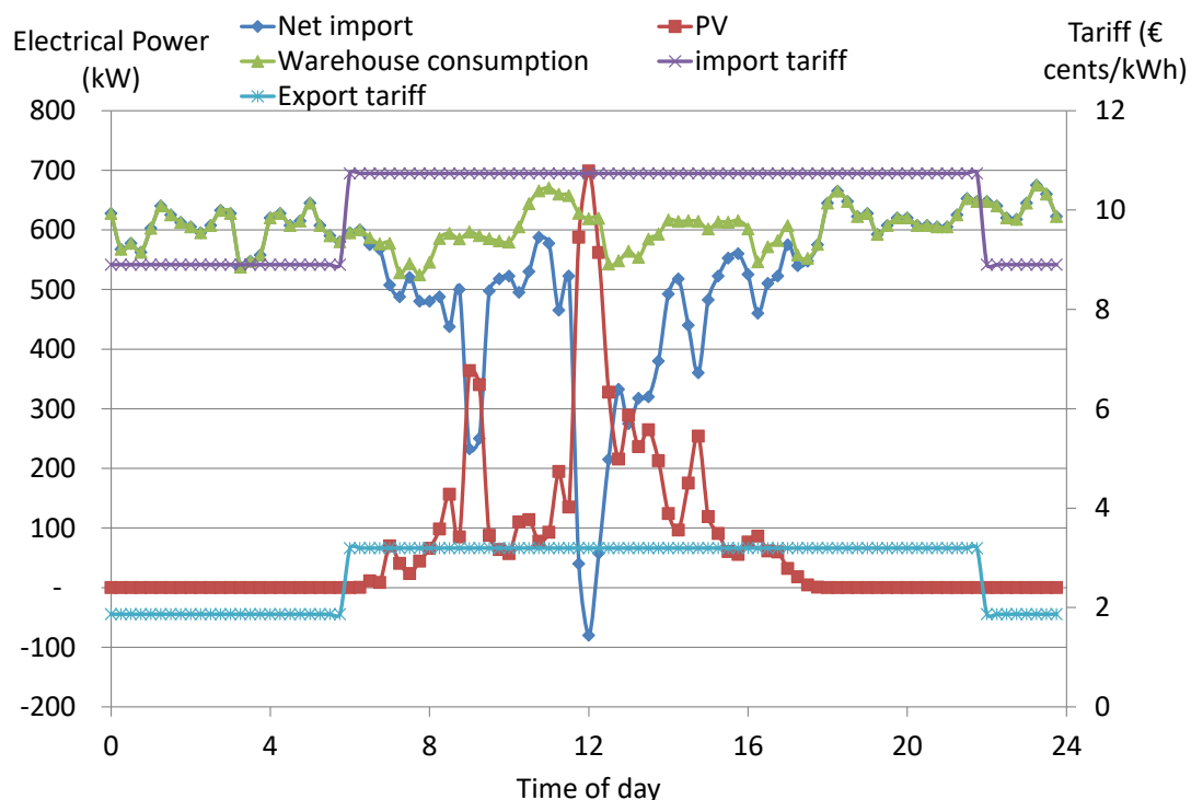
Figure 5. Electricity consumption, PV generation and tariffs at Belgium cold store.
