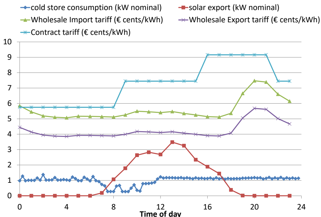
Figure 4. Electricity consumption, PV generation and tariffs at Spanish cold store.
